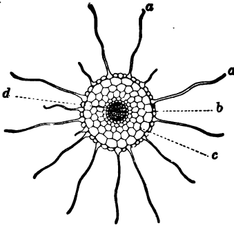
Cross section of a young taproot; a, a, root hairs; b, outer layer of bark; c, inner layer of bark; d, wood or central cylinder.
